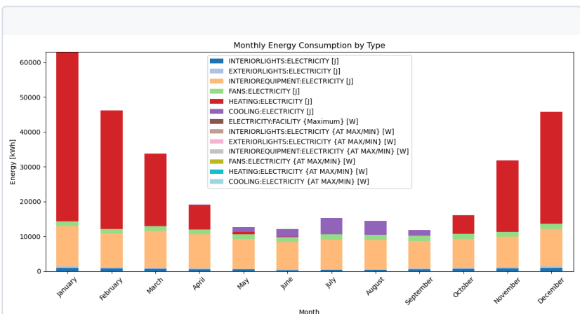
Figure — Disaggregated monthly profile by end use (OPE)
